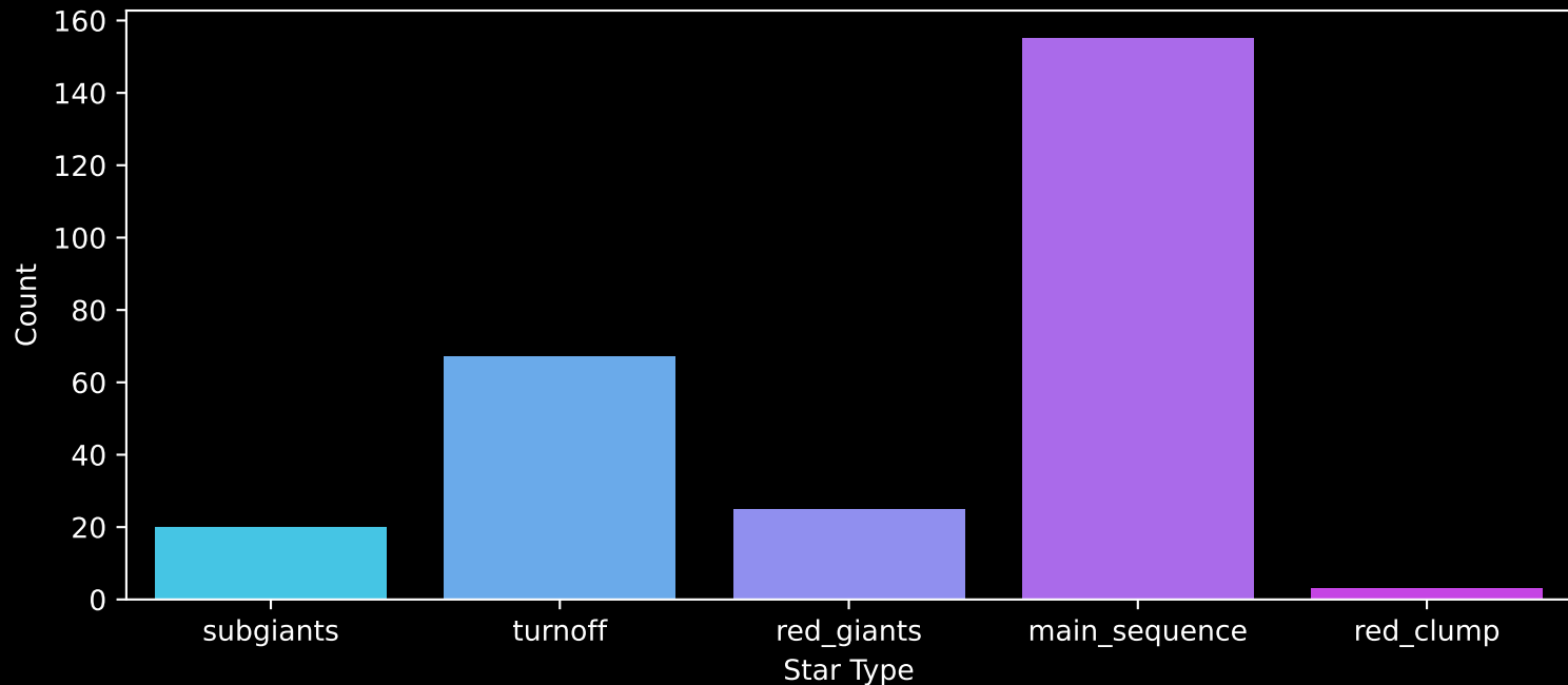
GALAH DR4 Field: [434] Count plot of Star Type
