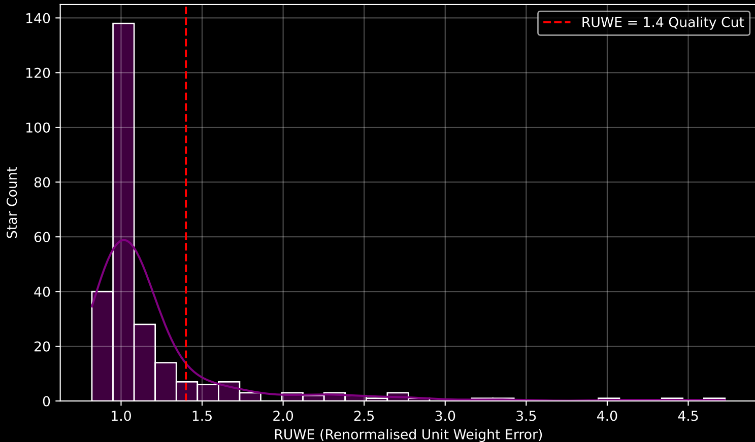
GALAH DR4 Field [434] RUWE Distribution (n= 263)
