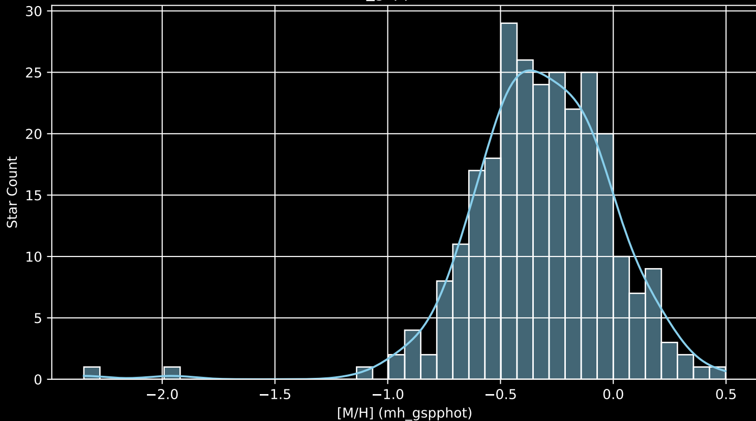
GALAH DR4 Field: [434] [M/H] (mh_gspphot) (n= 269)
