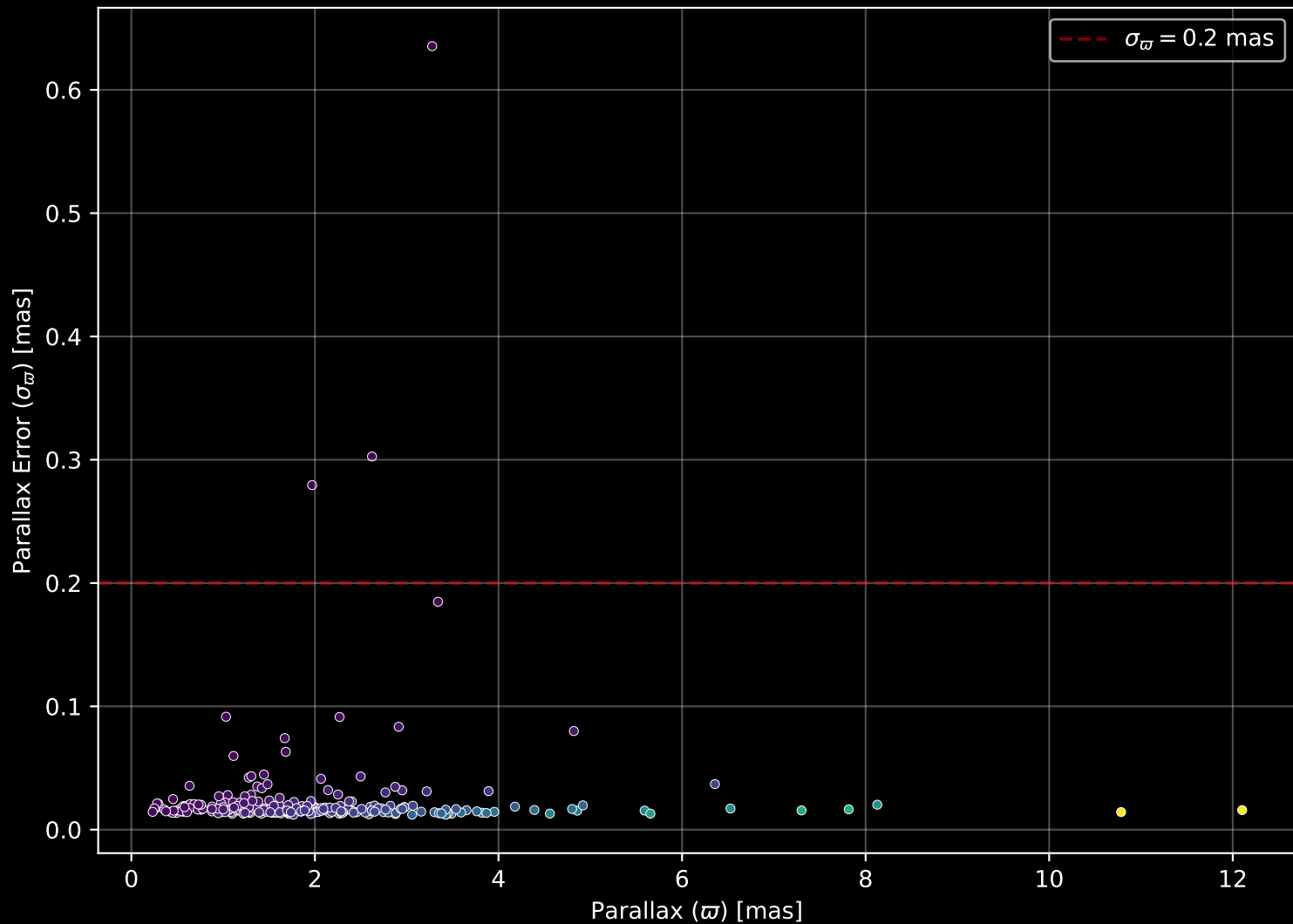
GALAH DR4 Field: [434] Parallax Quality (n= 270)
