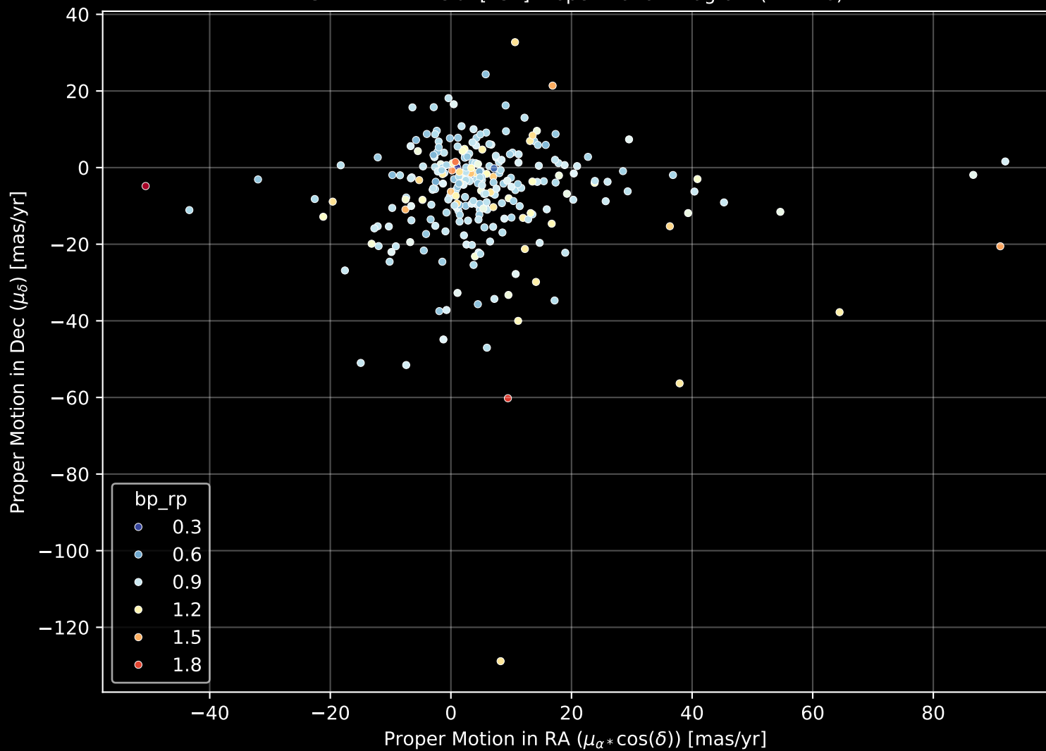
GALAH DR4 Field: [434] Proper Motion Diagram (n= 270)
